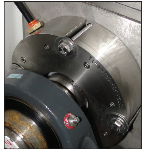
The AM Food Grade is a permanent shaft seal made of food grade materials for applications in the food processing industry.
