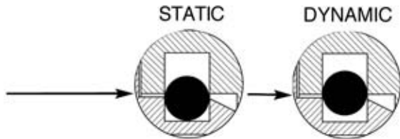
The Inpro/Seal® "VBX" Bearing Isolator, with its unique internal O-ring, provides an effective vapor barrier.
